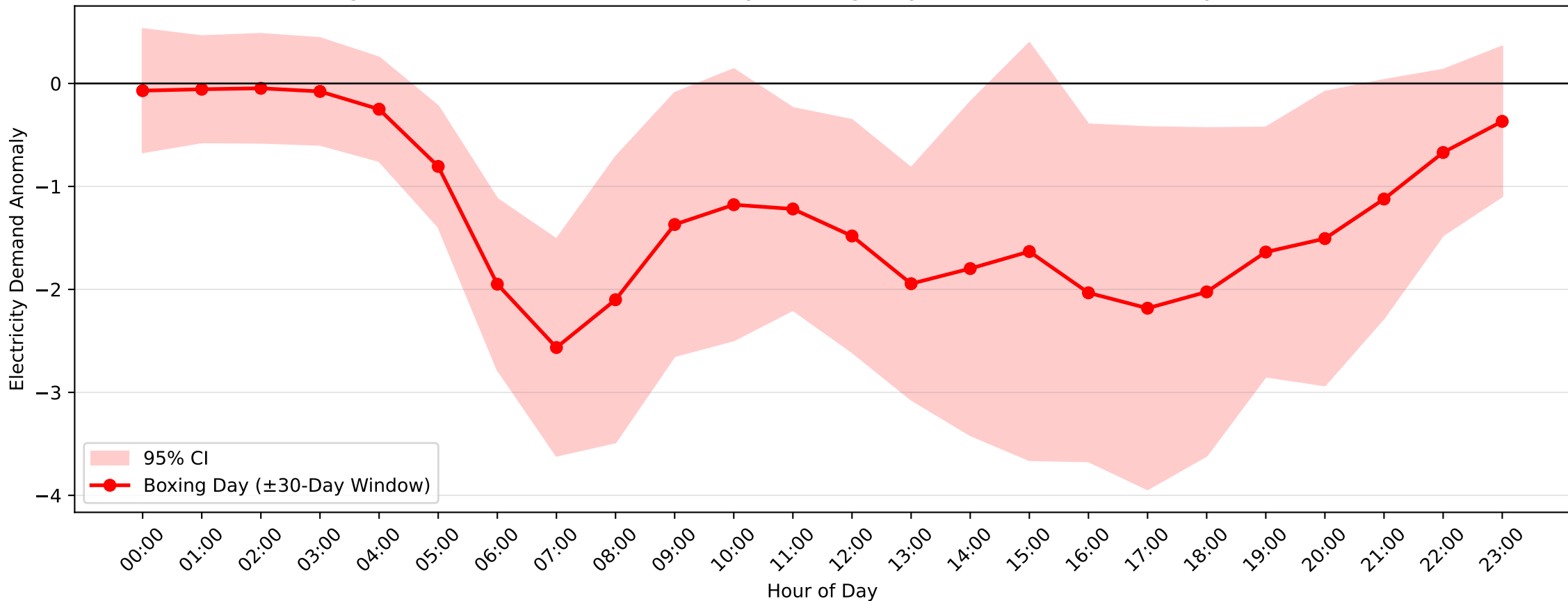
Balgowlah North Demand Anomaly: Boxing Day (2004-2017, \pm 30 -Day Window)
